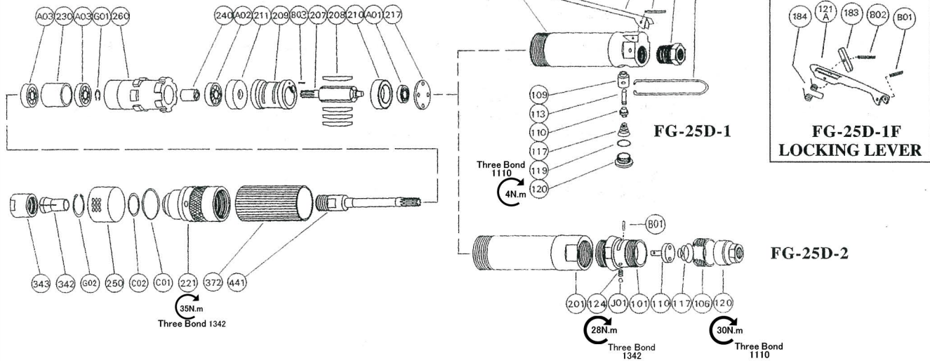
FG-25D-1, -1F ,-2
